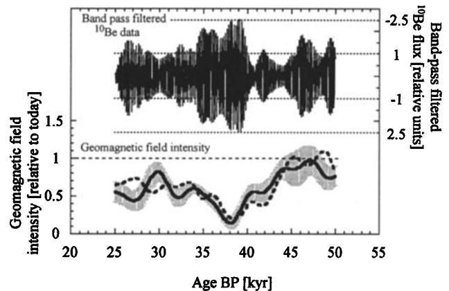
Figure 4. Upper panel: Band pass filtered ^{10}\text{Be} flux [ (215 \text{ yr})^{-1} \leq \tau \leq (195 \text{ yr})^{-1} ] [ Paillard et al. , 1996] over the time period of 25 to 50 kyr BP. Lower panel: paleomagnetic field intensities during the last ice age: The first (dotted line) is derived from remanence measurements of several Mediterranean sediment cores [ Tric et al. , 1992]. The second (solid line) is based on remanence measurements of several North Atlantic sediment cores [ Laj et al. , 2000]. The shaded area corresponds to the \pm 2\sigma uncertainties. Both records are low pass filtered (cut off frequency = 1/3 \text{ kyr}^{-1} ) to obtain a comparable time resolution as the envelope of the band pass filtered ^{10}\text{Be} flux.
