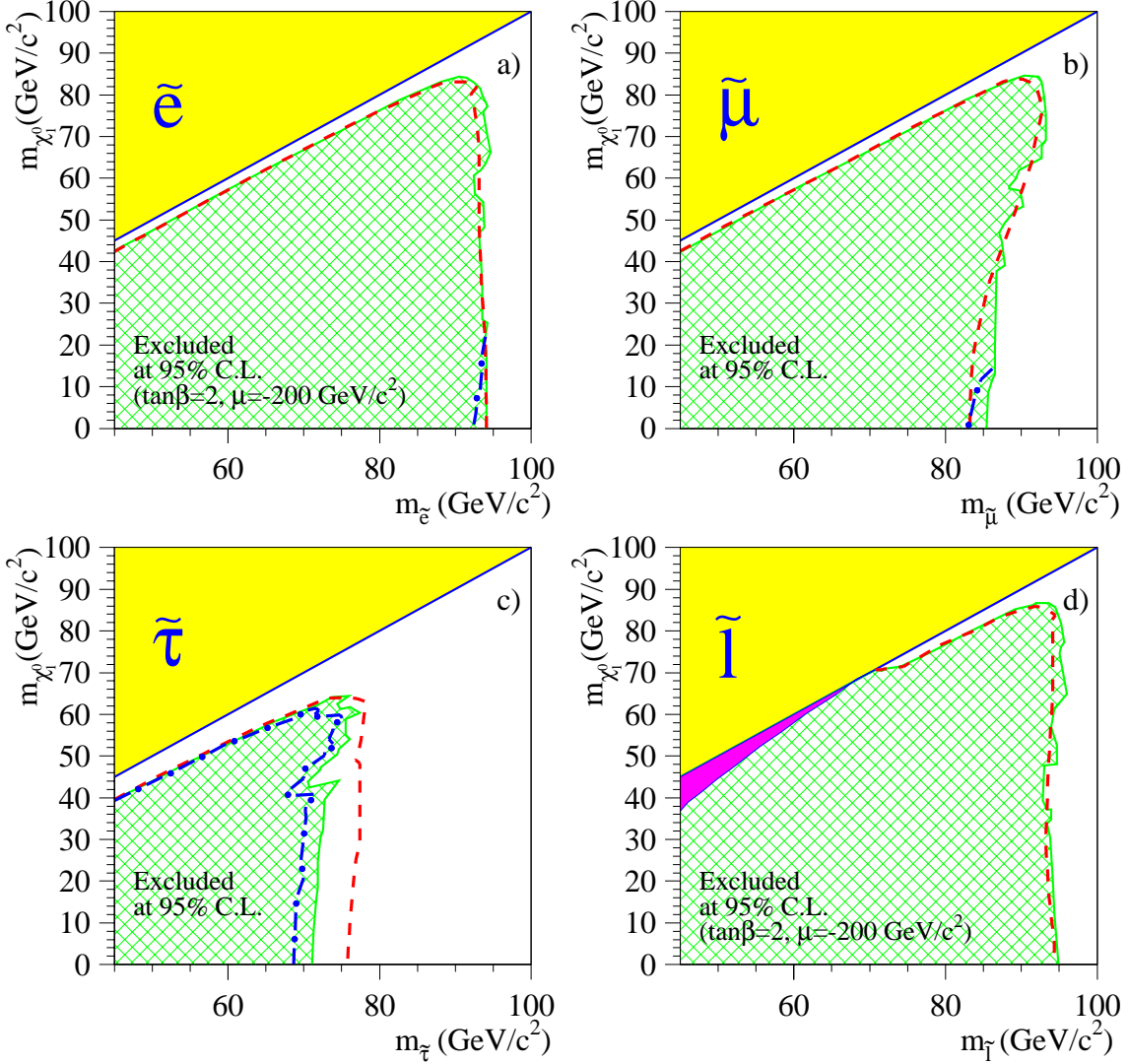
Figure 1: Excluded regions at 95% C.L. in the m_{\tilde{\ell}_R} vs m_{\chi_1^0} plane from slepton searches assuming \text{BR}(\tilde{\ell} \rightarrow \ell\chi_1^0) = 100\% (cross-hatched regions); the dashed curves show the expected exclusion under the same assumptions. The dot-dashed curves in a) and b) show the effect of cascade decays for \tan\beta = 2 and \mu = -200 GeV/c 2 , assuming zero efficiency for those decays. The dot-dashed curve in c) shows the limit in the case of minimal \tilde{\tau}_1\tilde{\tau}_1 Z coupling. In d) , the effect of cascade decays is included. The dark shaded region is not accessible because the common scalar mass at the GUT scale becomes unphysical. In all the plots, the light shaded region corresponds to the m_{\tilde{\ell}} < m_{\chi_1^0} disallowed region.
