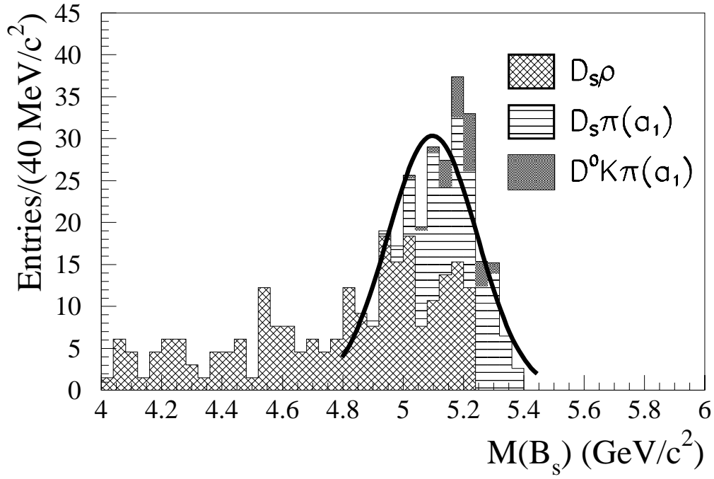
Figure 2: The Monte Carlo composition of the satellite peak including the effects of experimental resolution. The notations in the plot are the following: D_s \rho corresponds to D_s^- \rho^+ and D_s^{*-} \rho^+ decay channels of the B_s^0 ; D_s \pi(a_1) corresponds to D_s^{*-} \pi^+ and D_s^{*-} a_1^+ ; D^0 K \pi(a_1) shows the contribution from \bar{D}^{*0} (2007)^0 K^- \pi^+ and \bar{D}^{*0} (2007)^0 K^- a_1^+ decay channels. All contributions have been normalised according to the evaluation of the branching fractions discussed in Section 3.1 and including reconstruction efficiencies evaluated using simulated events.
