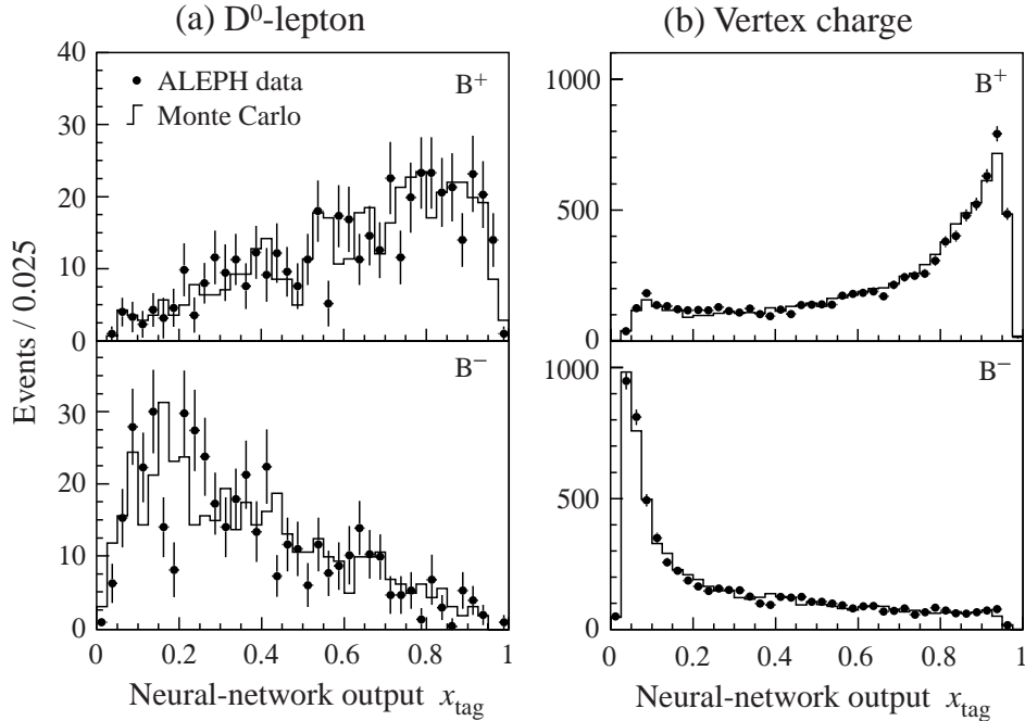
Figure 7: Production-state tag neural-network output for (a) \bar{D}^0\ell^+ and (b) vertex-charge selected samples. In each figure the upper plot is for events selected as B^+ candidates, the lower for B^- .
