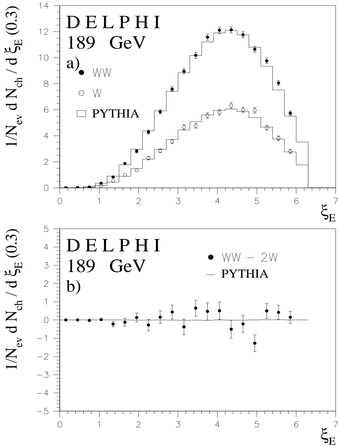
Figure 4: (a) Corrected \xi_E distributions of charged particles for (4q) events (closed circles) and (2q) events (open circles), at 189 GeV, compared to simulation without colour reconnection. The difference between (4q) and twice (2q) is shown in (b).
