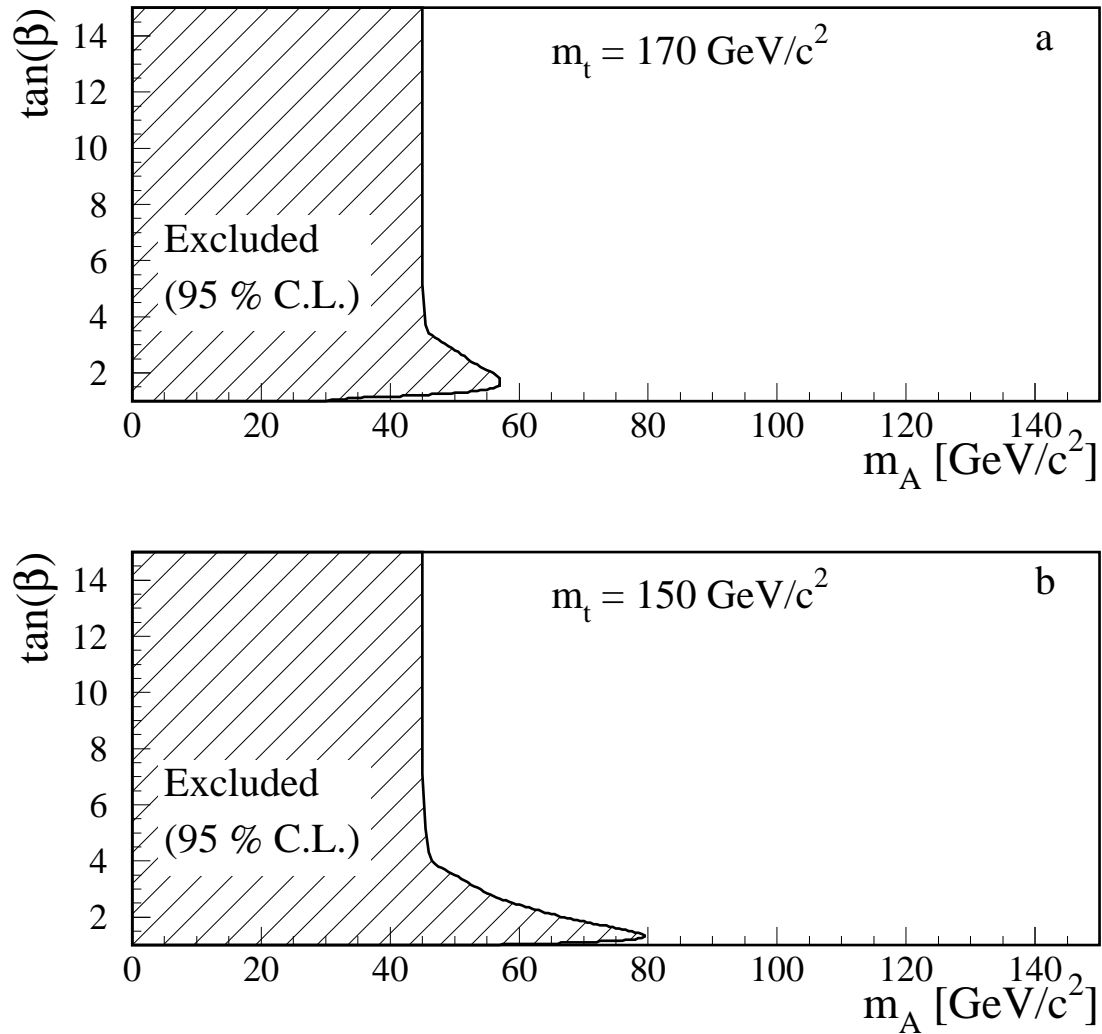
Figure 7: \tan\beta/m_A limit contour (at 95 % confidence level) obtained from searches for hA and hZ^* channels in the MSSM case with m_{sg} = 1 TeV/c 2 . The two figures correspond to: (a) m_t = 170 GeV/c 2 and (b) m_t = 150 GeV/c 2 . The one-loop formulae of reference [2] were used.
