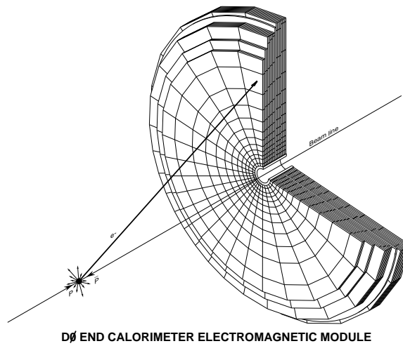
FIG. 7. The ECM section of an end calorimeter.
