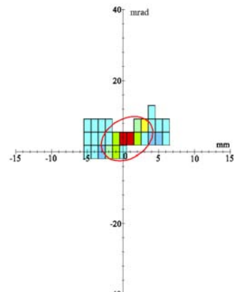
Fig. 8 : I=50 nA, (0.85xI) in \nu = 13 .mm.mrad
