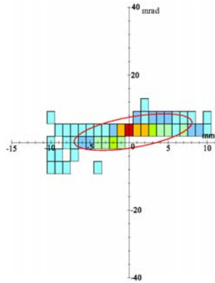
Fig. 6 : I=100 nA, (0.87xI) in \nu = 25 .mm.mrad
