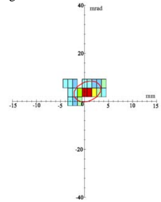
Fig. 10 : I=32 nA, (0.88xI) in \nu = 12 .mm.mrad
