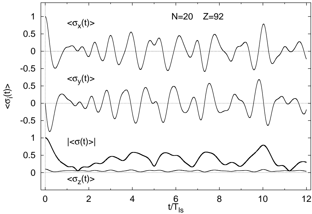
Figure 5. Time evolution of the average values of spin components \langle \sigma_i \rangle , i = x, y, z for system with N = 20 , Z = 92 .
