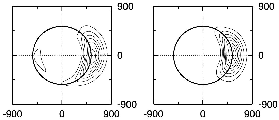
Figure 9. The best revival of the WP for the system with N = 20 , Z = 92 presented on the plane of the classical orbit. The time instant t = 10.063545 T_{Is} corresponds to the highest value of the autocorrelation function displayed in Fig. 3. For comparison with the spin components at t = 0 see the upper row of the Fig. 7
