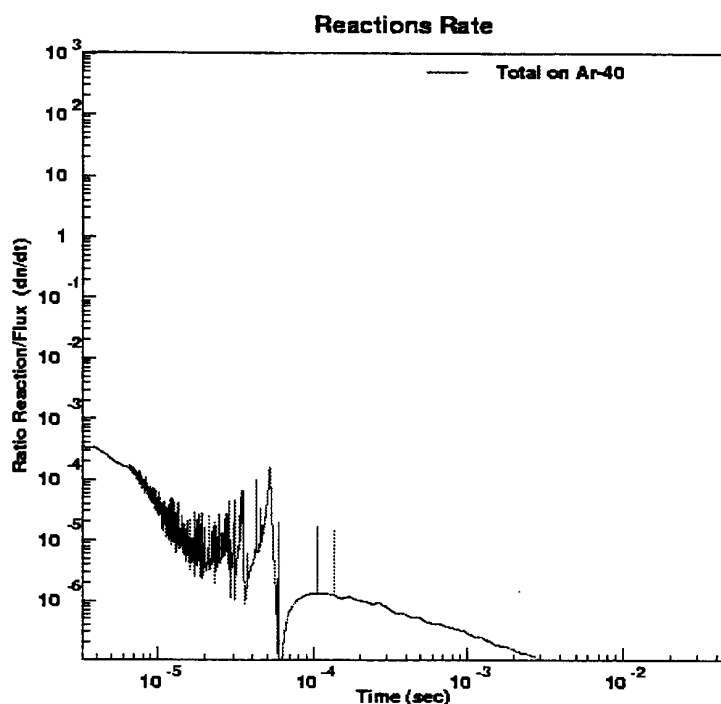
Figure 5.13: Relative Event Rates in 4 mm Argon at 2 bars over 1000 cm 2 surface.
