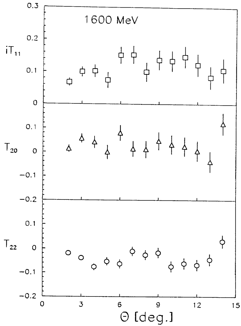
Fig. 6. Analyzing powers iT_{11} , T_{20} , T_{22} at 1.6 GeV.
