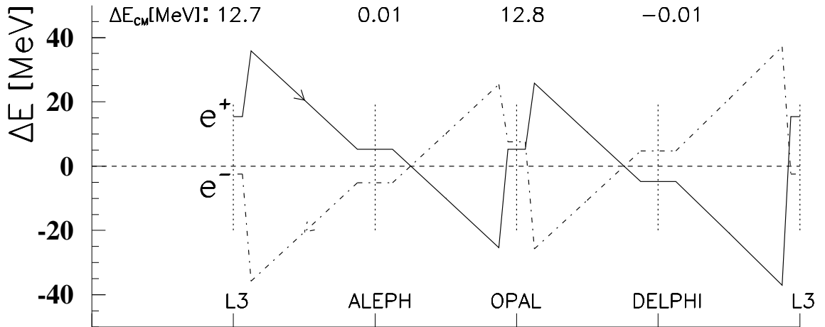
Figure 3: Deviation of particle energies from the average beam energy as a function of the position in LEP, for typical 1991 running conditions. The gain in energy on the left-hand side of the L3 experiment is larger due to additional super-conducting cavities. The numbers ' \Delta E_{CM}[\text{MeV}] ' indicate the deviation of the centre-of-mass energy at the interaction points.
