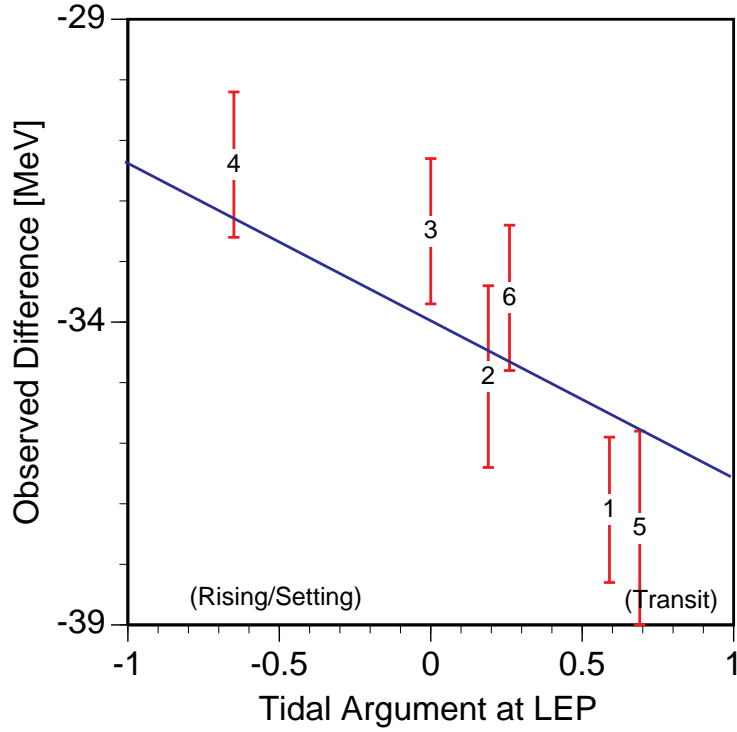
Figure 2: Deviations of the beam energy from the field display value as observed from beam energy measurements with the technique of resonant depolarization. The x-axis represents the tidal force exerted by the Moon and the Sun, normalized between -1 and 1; -1 corresponds to rising or setting of the Moon. The numbering on the measurements represents their sequence in time, and the error bars give the range in beam energy within which resonant depolarization was observed.
