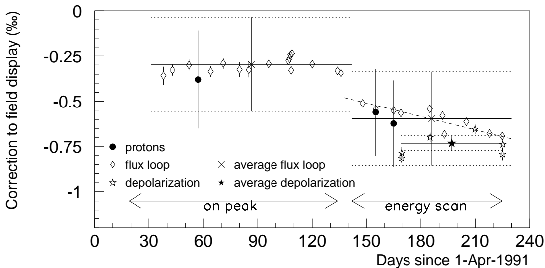
Figure 1: Beam energy calibrations in 1991.
