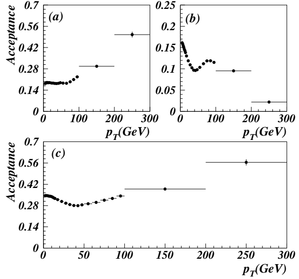
FIG. 10. Final acceptance as a function of p_T for (a) the CCC, (b) CCEC event topologies, and (c) for the combined event sample.
