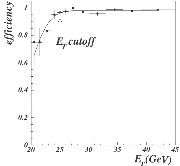
FIG. 2. Electron detection efficiency as a function of electron E_T at the trigger level. The efficiency is essentially flat above our final E_T cutoff of 25 GeV.
