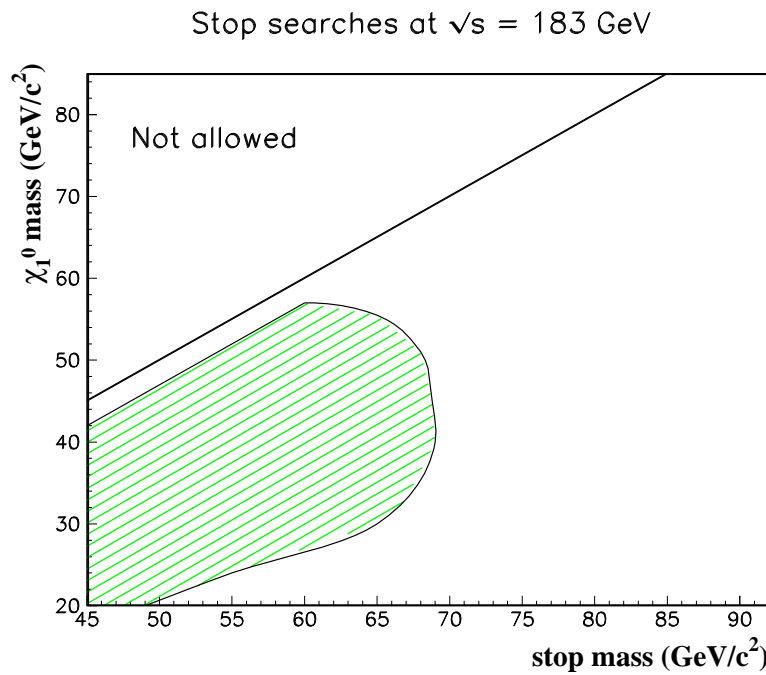
Figure 13: Stop indirect decay with \lambda coupling: exclusion domain in m_{\tilde{\chi}_1^0} versus m_{\tilde{t}_1} for the \tilde{t}_1 pair production in case of maximal decoupling to the Z boson; the diagonal line separates the plot into two regions: in the upper part, no R_p decay of \tilde{t} is allowed; in the lower part, the indirect decay into c\tilde{\chi}_1^0 is allowed, so the excluded area (hatched part) depends on the neutralino mass.
