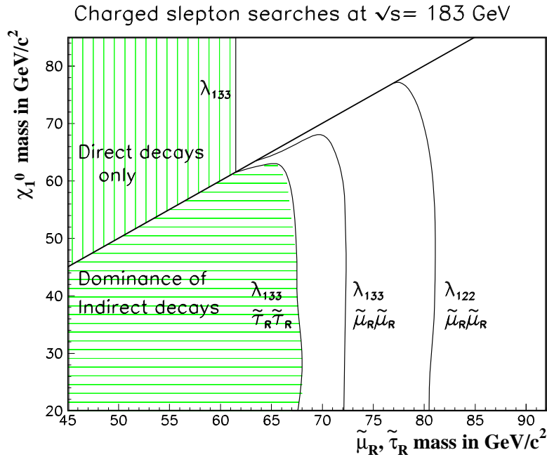
Figure 12: Slepton search with \lambda coupling: exclusion domain in m_{\tilde{\chi}^0_1} versus m_{\tilde{l}} for the \tilde{l} pair production cross-section; the diagonal line separates the plot into two regions: in the upper part, only the direct decay is allowed; in the lower part, the indirect decay is dominant, so the exclusion limit depends also on the neutralino mass. The limit is given by the direct decay.
