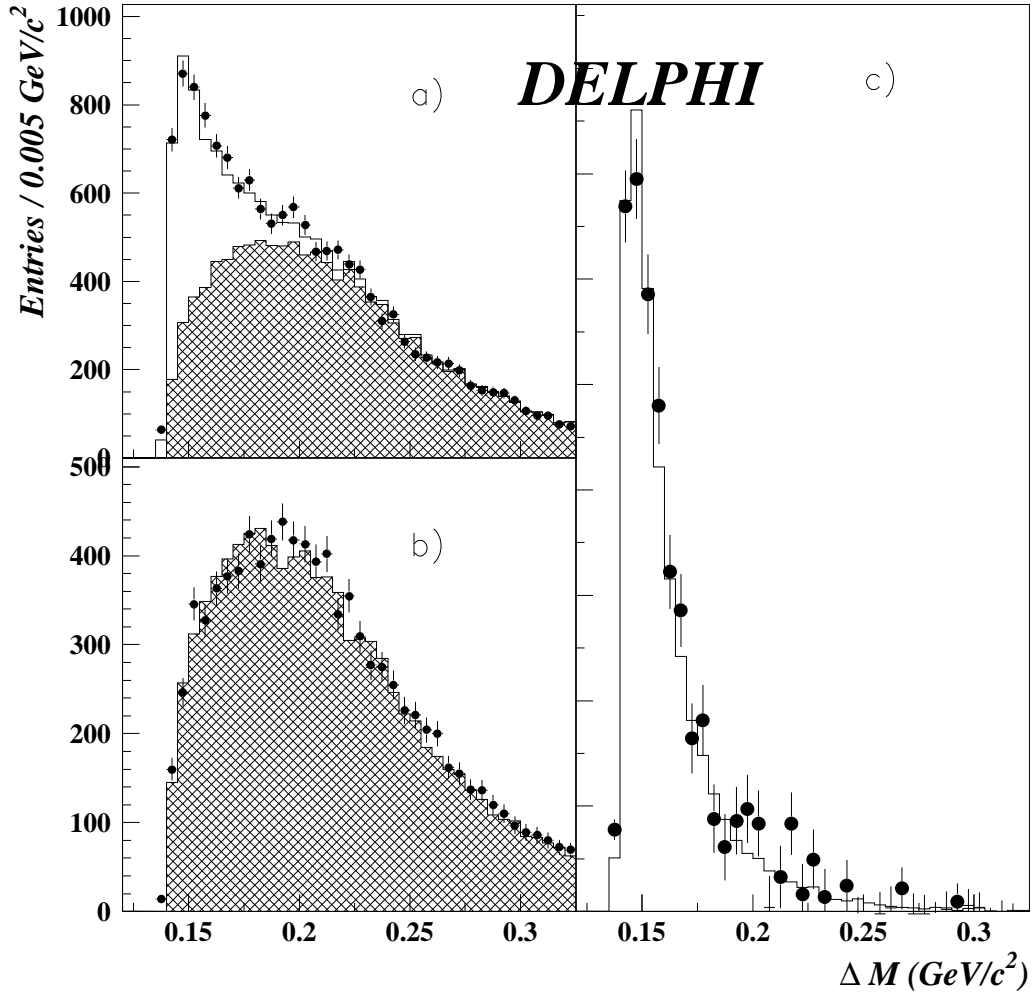
Figure 7: \Delta M = M_{D^{*-}} - M_{D^0} distribution for the inclusive analysis, when the lepton and the \pi^* have a) opposite charge and b) same charge. The dots are the data, the shadowed area shows the prediction of the simulation for the combinatorial background. The experimental distribution, after subtraction of the simulated background, is compared to the sum of all expected D^{*-} sources in c).
