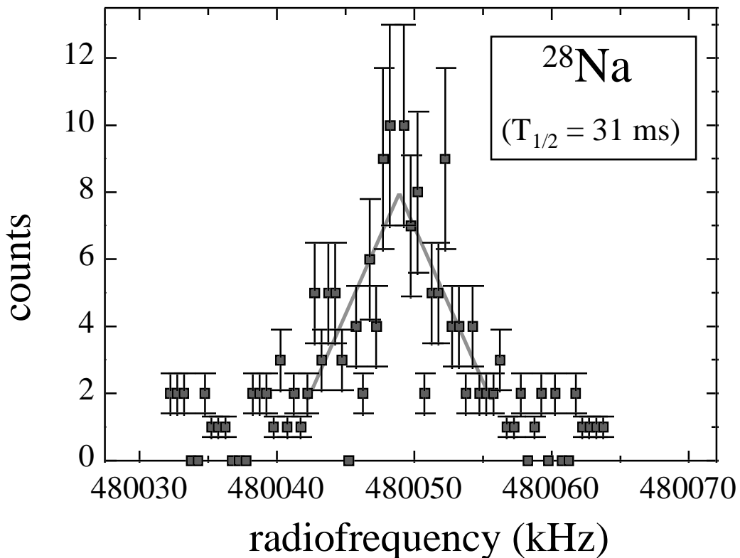
FIGURE 2. A recorded (reconstructed) peak for ^{28}\text{Na} ( T_{1/2} = 30.5 ms). This measurement corresponds to 64 (random) frequency steps of 320 ms each. The center frequency of about 480,050 kHz is derived from a triangular fit [15] and corresponds to harmonic number 2342 of the cyclotron frequency of ^{28}\text{Na} in the 0.37359 T field at a beam energy of 60 keV. The mass resolution is 47,860.
