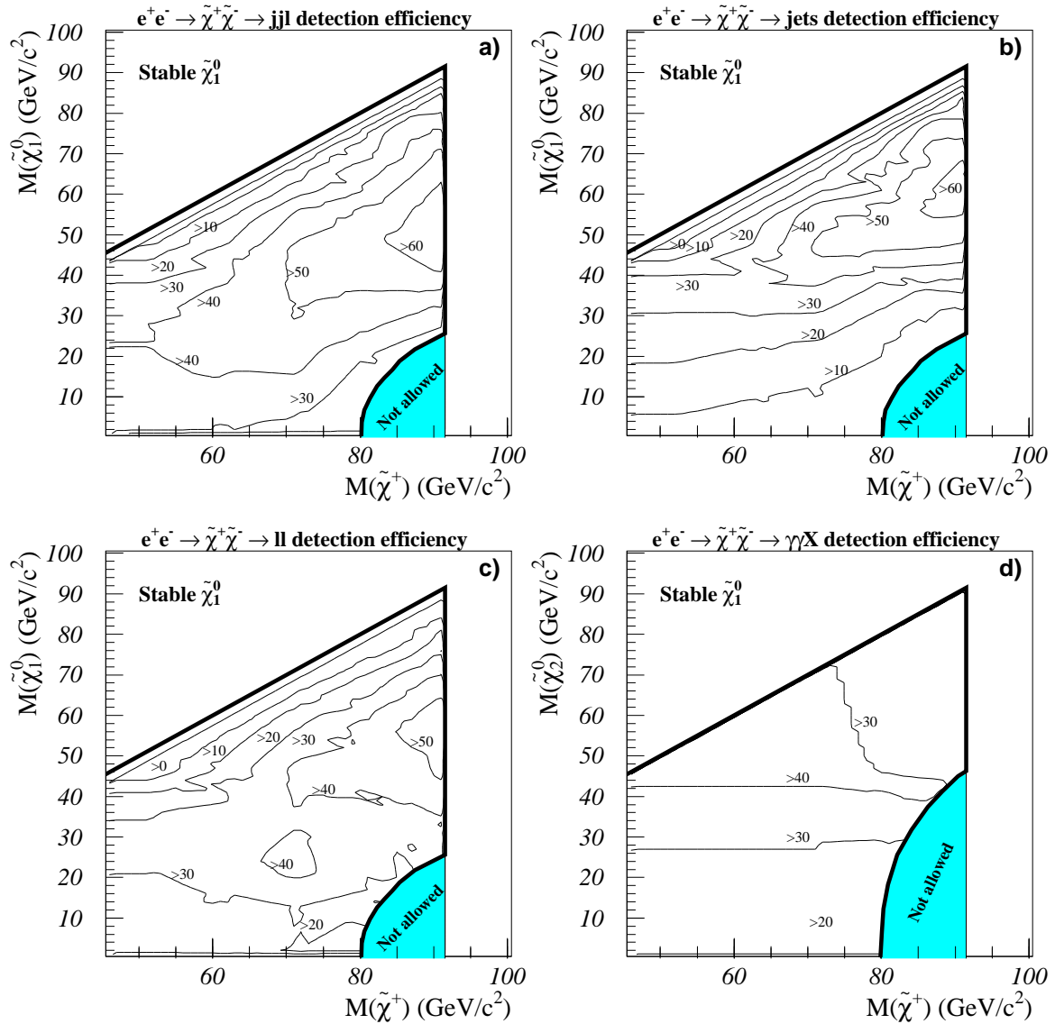
Figure 2: Chargino pair production detection efficiencies (%) for the 4 topologies a) jj\ell , b) \text{jets} , c) \ell\ell and d) \gamma\gamma X , at 183 GeV in the (M_{\tilde{\chi}^\pm}, M_{\tilde{\chi}^0}) plane. A stable neutralino is assumed.
