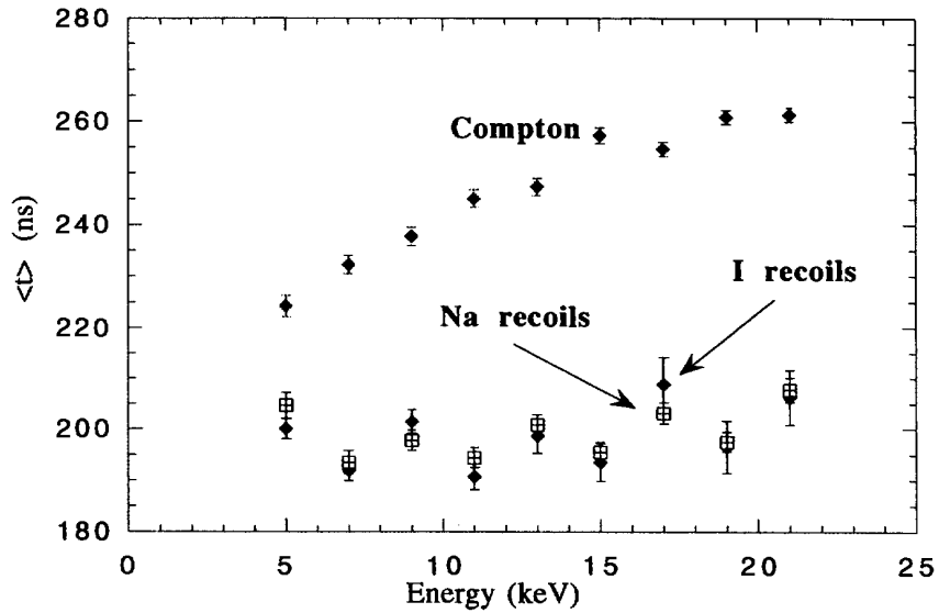
Figure 9: Variation of the mean \langle t \rangle variable for the Sodium, Iodine recoils and Compton populations (neutron beam, 1" by 1" crystal).
