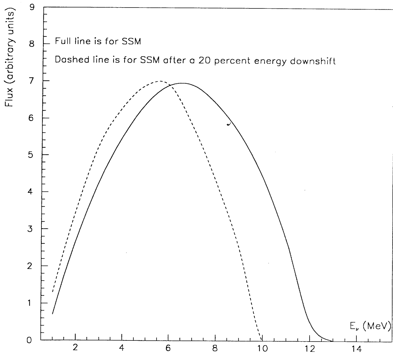
Fig.2 Energy spectrum of the ^8\text{B} neutrinos
