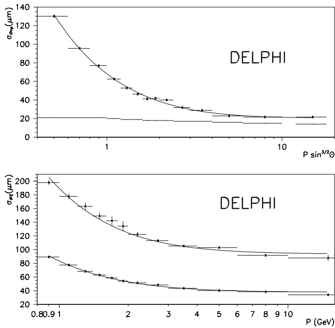
Figure 13: Upper: Mean track extrapolation uncertainty in R\phi measured as a function of p \sin^{3/2}\theta ( p in \text{GeV}/c ). The values are determined by subtracting quadratically the vertex position uncertainty, shown by the bottom curve, from the measured impact parameter uncertainty. The full line depicts (65/p \sin^{3/2}\theta \oplus 20) \mu\text{m} . Lower: Mean track extrapolation uncertainty in the Rz plane, measured similarly as a function of the particle momentum. The two curves correspond to tracks with 80^\circ < \theta < 90^\circ (bottom) and 45^\circ < \theta < 55^\circ (top). The full lines depict (71/p \oplus 39) \mu\text{m} and (151/p \oplus 96) \mu\text{m} respectively.
