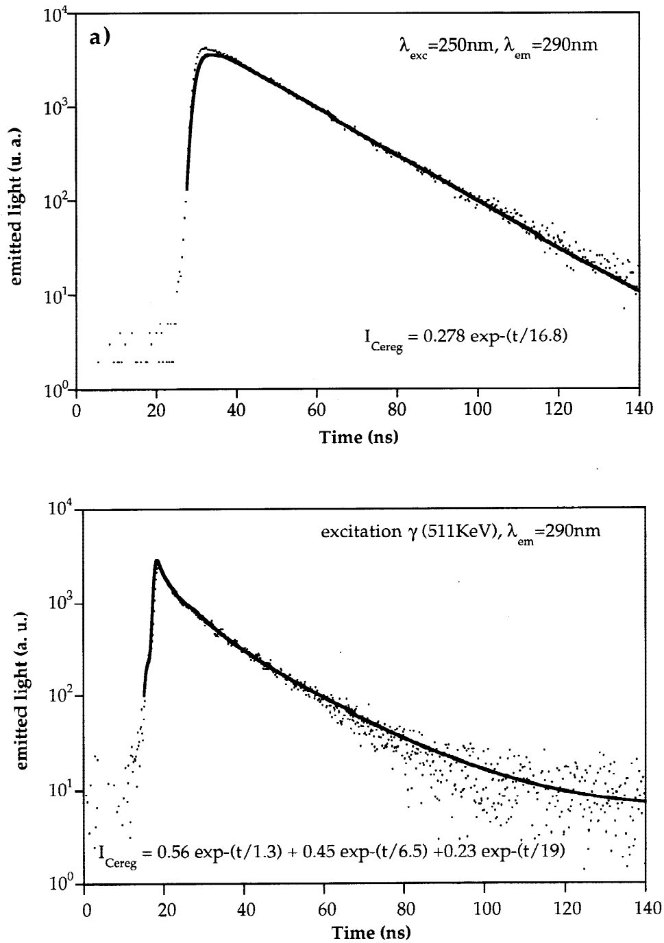
Fig. 9: Decay curves for \text{Ce}^{3+} ion in regular site (CF557 from Optovac): a) under direct 250nm excitation; b) under gamma excitation. The coefficient of the exponentials in the formula are obtained by deconvoluting the instrumental response from the experimental curve; instrumental response is not given in figure
