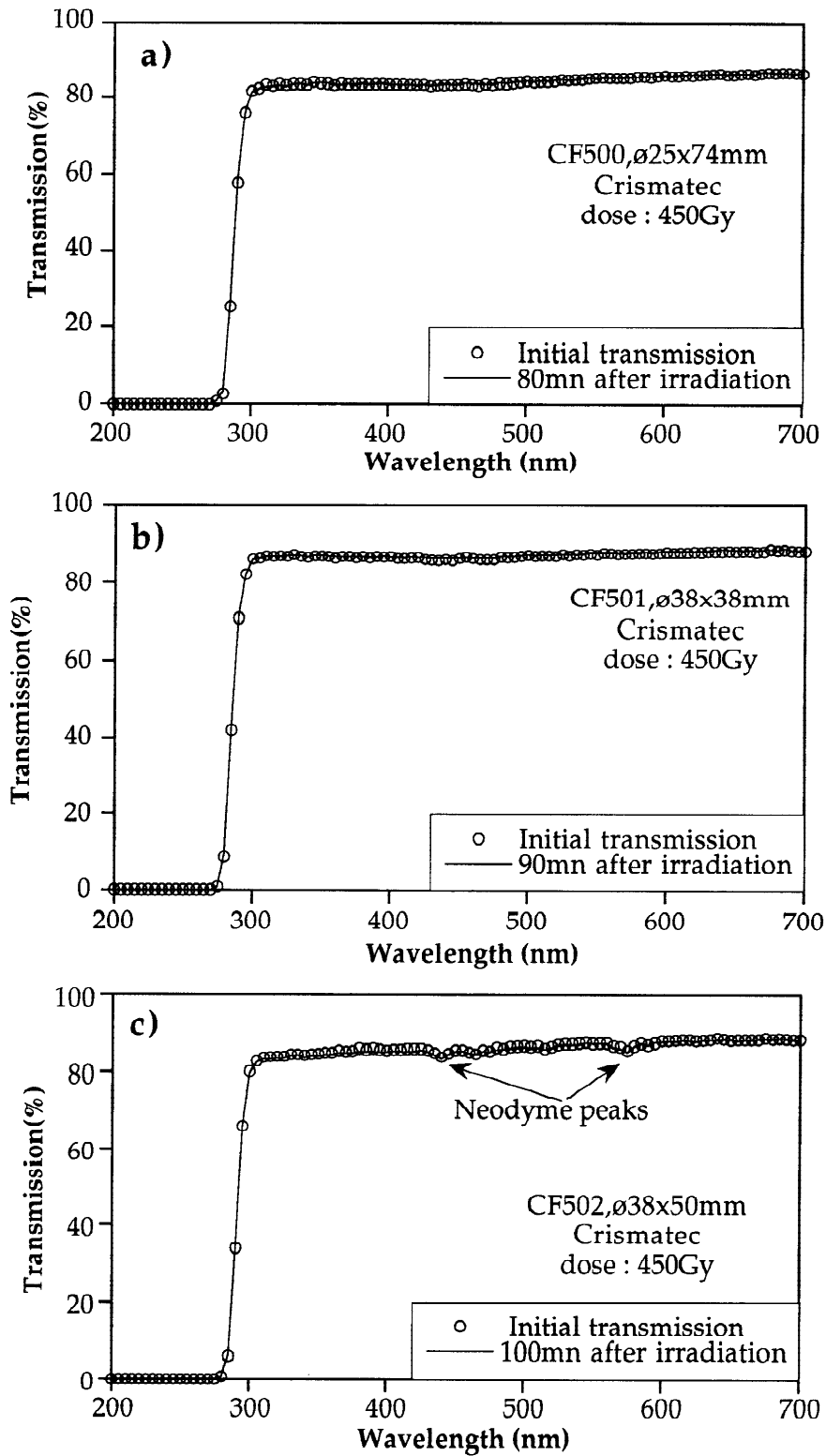
Fig. 14: Effects of radiations on several crystals (from Crismatec) after 500 Gy irradiation 60 Co
