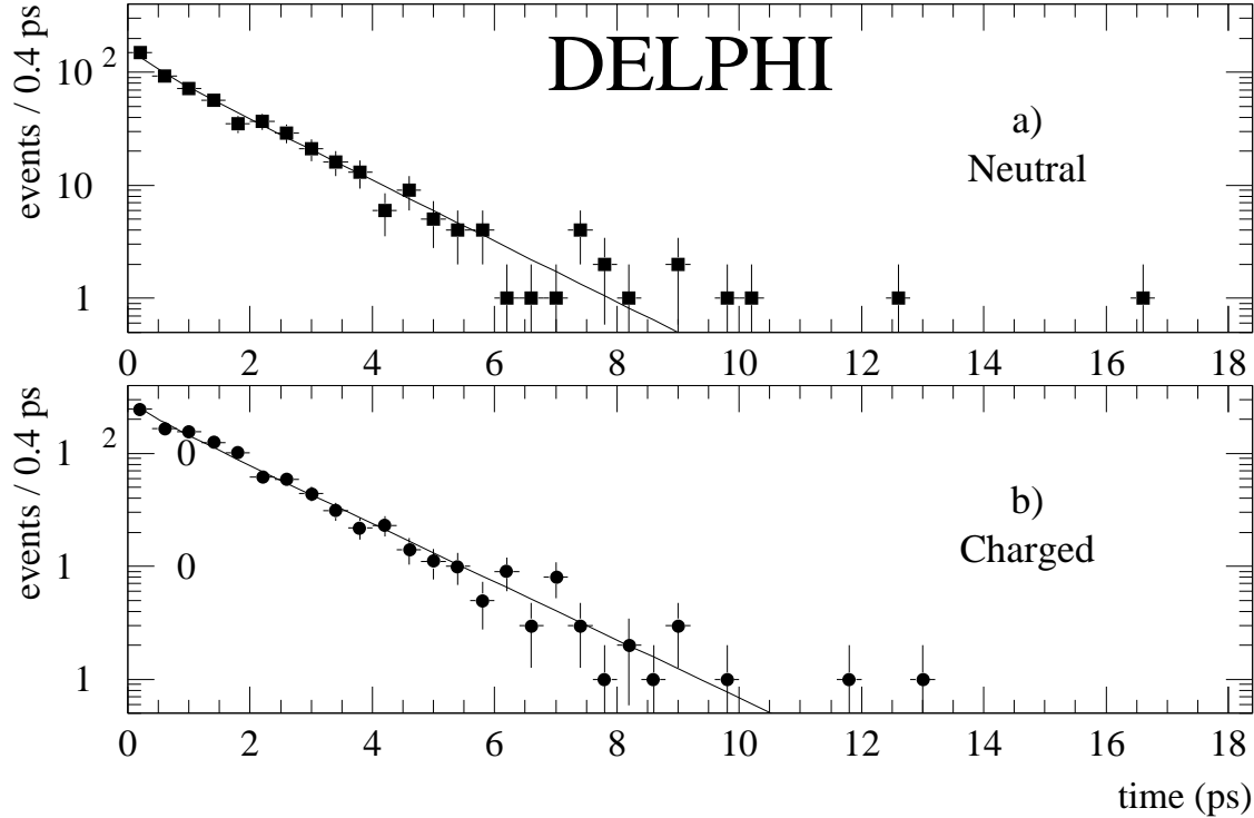
Figure 6: The excess proper time distributions of the charged and neutral vertices, with the fit result superimposed. The slight curvature is because the fit is a sum of exponentials.
