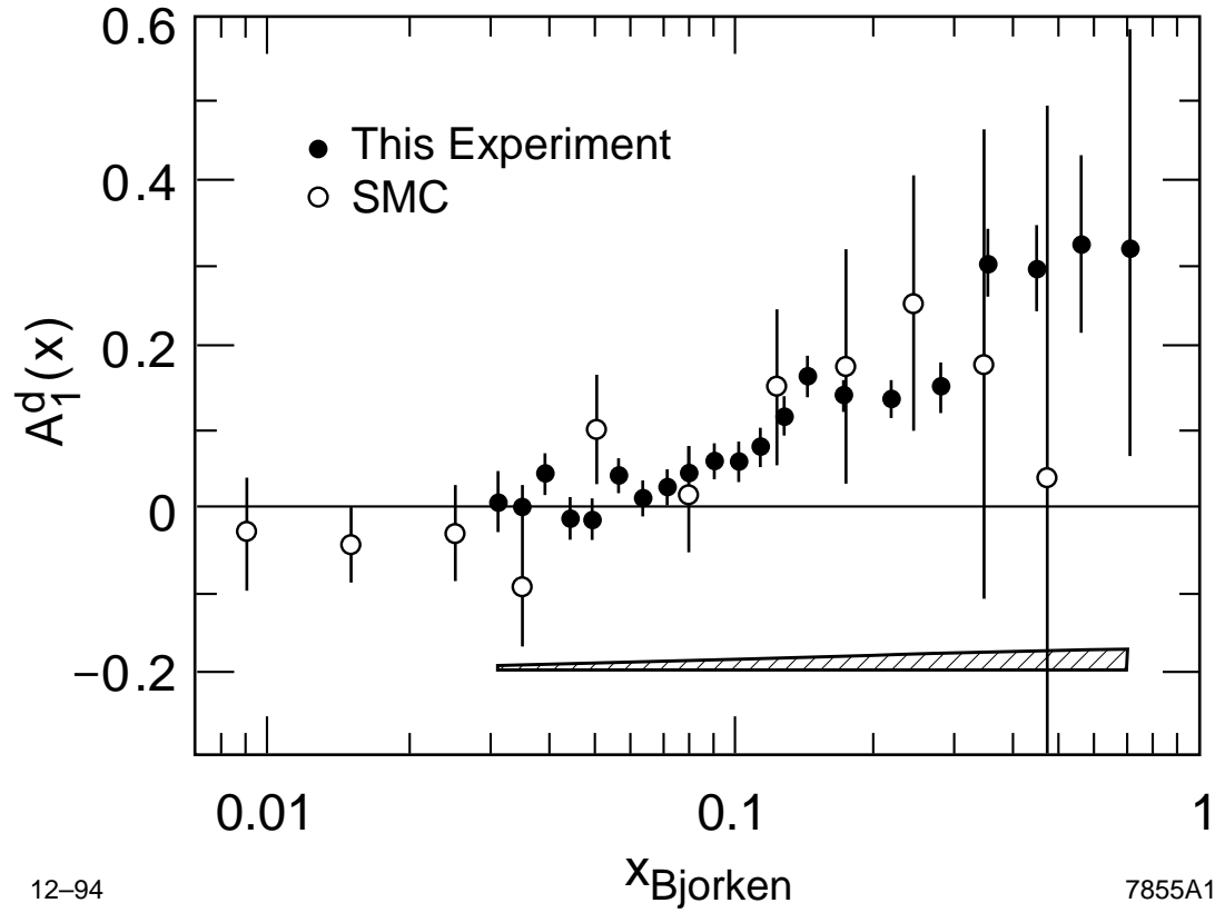
FIG. 1. The virtual photon asymmetry A_1^d from this experiment. The systematic errors are indicated by the shaded band. The average Q^2 varies from 1.3 (\text{GeV}/c)^2 at low x to 9 (\text{GeV}/c)^2 at high x . Data from the SMC collaboration [6] are also shown.
