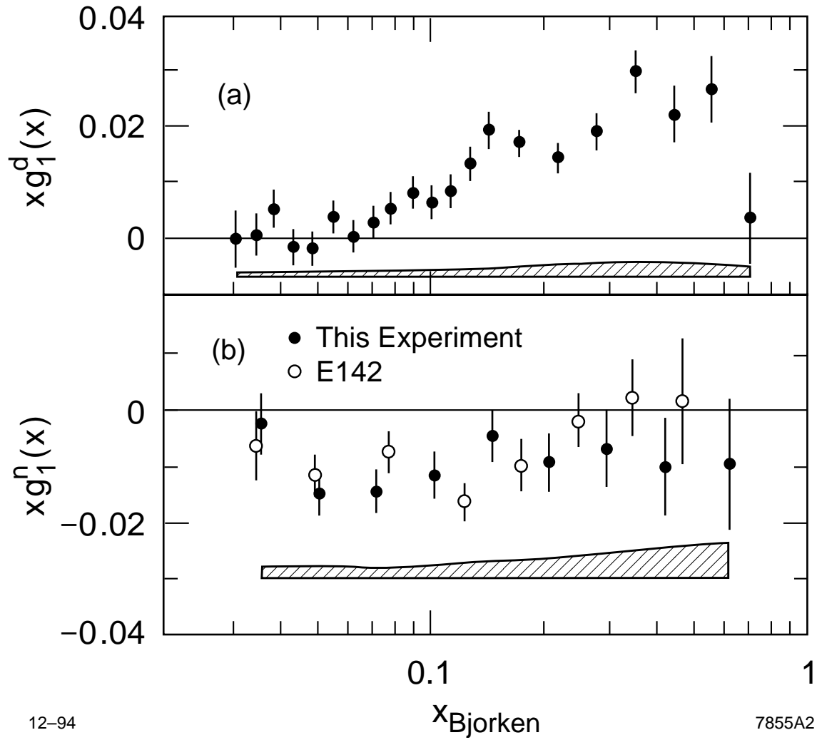
FIG. 2. Values of xg_1 from this experiment (E143) as a function of x for (a) the deuteron and (b) the neutron. The errors are statistical only. Systematic errors are indicated by the shaded bands. Also shown are the neutron results from SLAC E142. [5]
