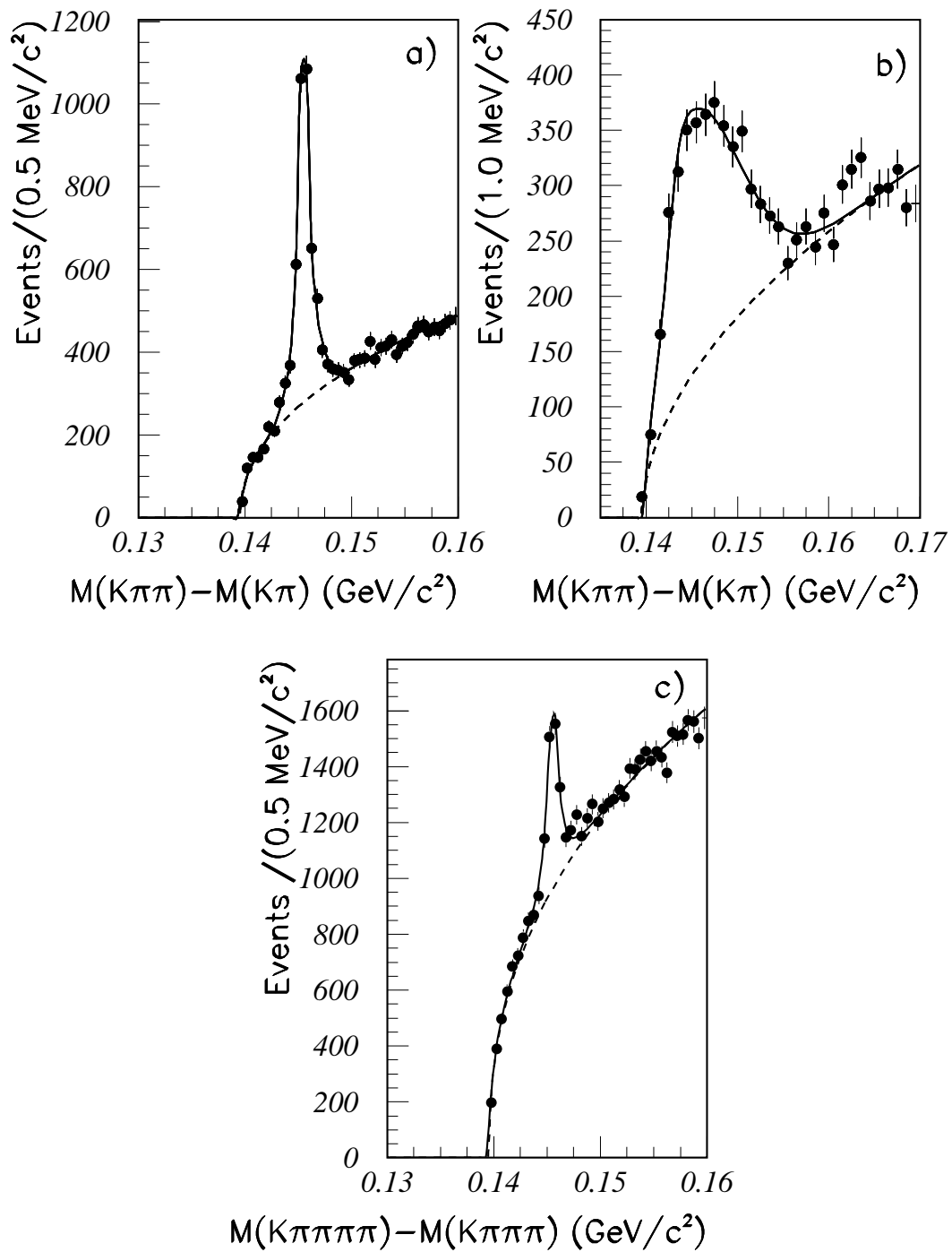
Figure 1: Distribution of \Delta M for a) K\pi , b) K\pi\pi^0 and c) K\pi\pi\pi D^0 decay candidates. The results of the fits, with signal and background shapes described in the text, are superimposed.
